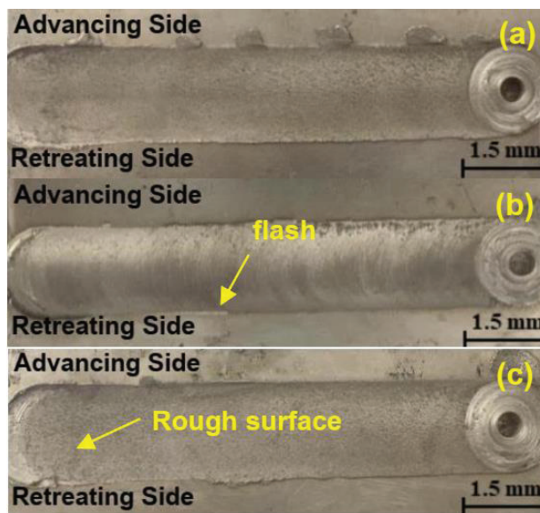
Figure 8 Characteristics of welding from top view surface using a square pin at rotation speed 2000 rpm and welding speed: (a) 80, (b) 112 and (c) 160 mm/min
