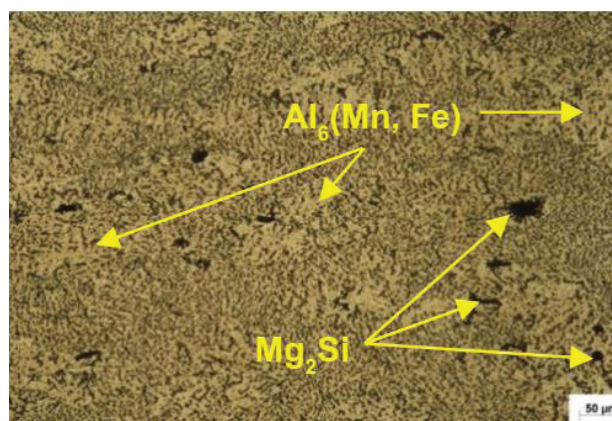
Figure 10 The base microstructure of AA 5083 aluminum Alloy
