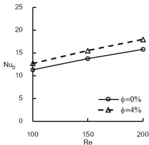
Figure 14 Stagnation point Nusselt number profiles for various Re numbers at H/B=2 and \phi=4\%
