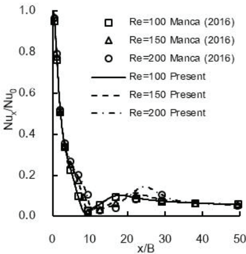
Figure 4 Validation of local Nusselt number Nu_x profiles are scaled with the stagnation point Nusselt number Nu_0 for H/B=4
