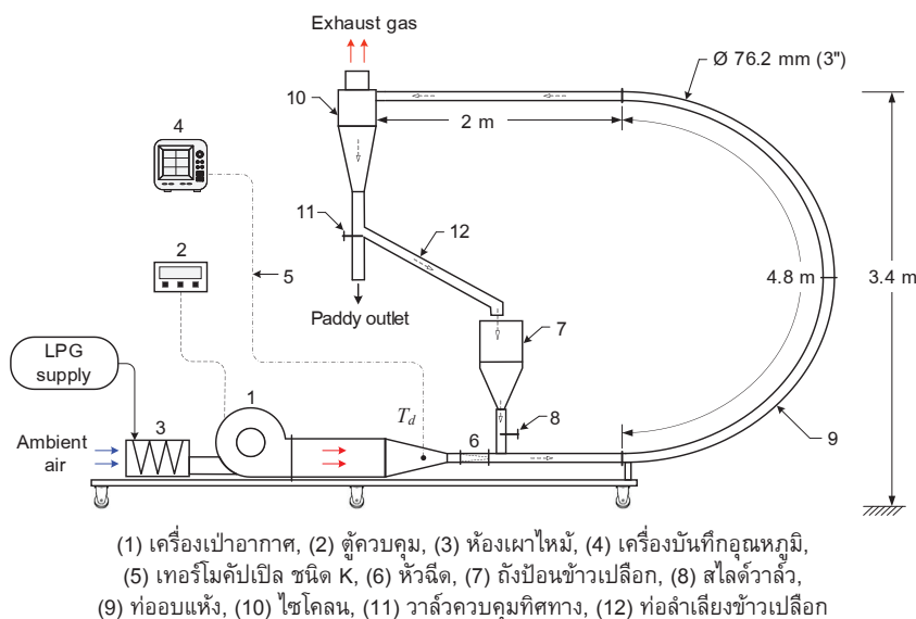
Figure 1 Schematic diagram of a pneumatic dryer with a curved drying pipe
