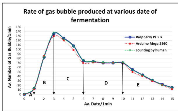
Figure 14 The average rate of carbon dioxide bubble generated from the fermentation process during the average period of 1-15 days/1minute at 25°C counted by the gas bubble counter controlled by Raspberry Pi3 B, Arduino mega 2560, and by human counting (Komorniczak, 2012)
