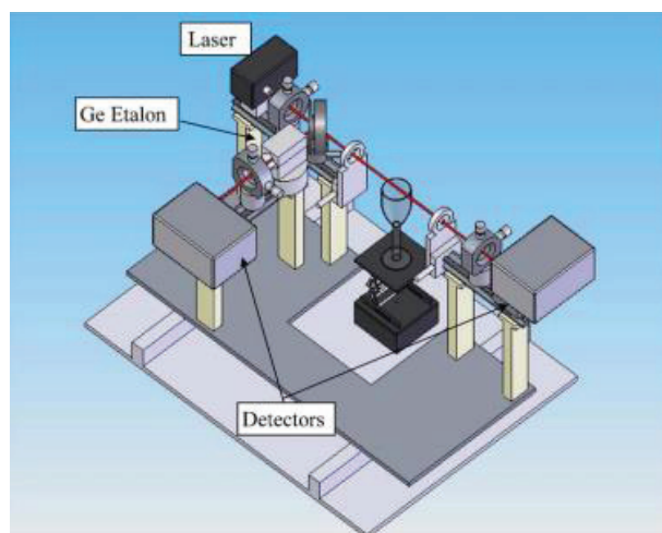
Figure 4 Experimental set up of CO 2 concentrations by infrared laser spectrometer. (Mulier et al. , 2009)
