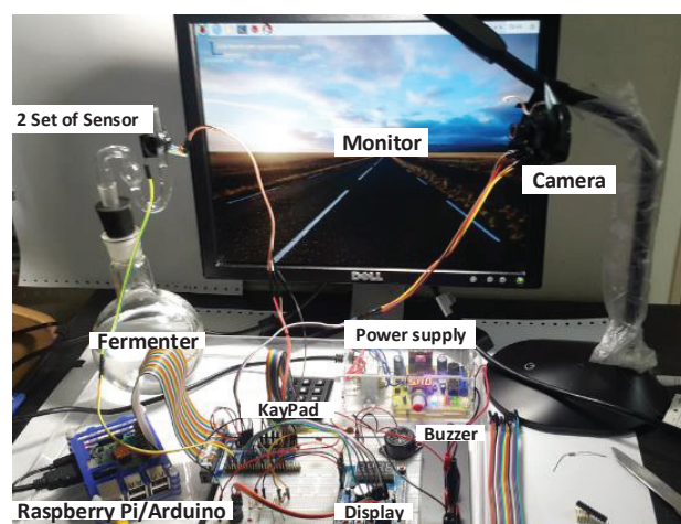
Figure 6 The structure of the gas bubble counter for the fermentation process (Wannaprapa, 2020)
