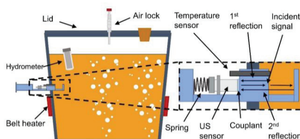
Figure 5 Experimental apparatus and measured US wave reflections (Bowler, et al. , 2021)
