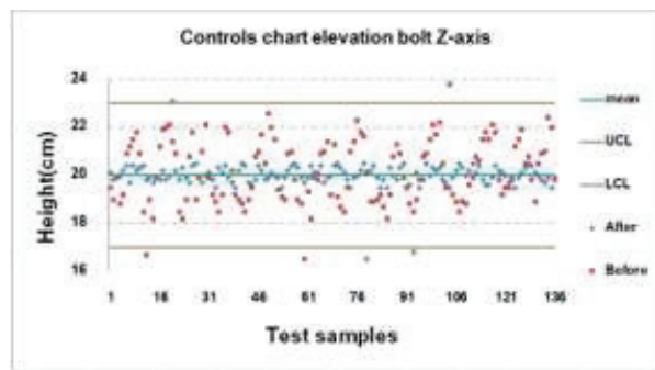
Figures 12 Control chart of elevation bolt in Z-axis
