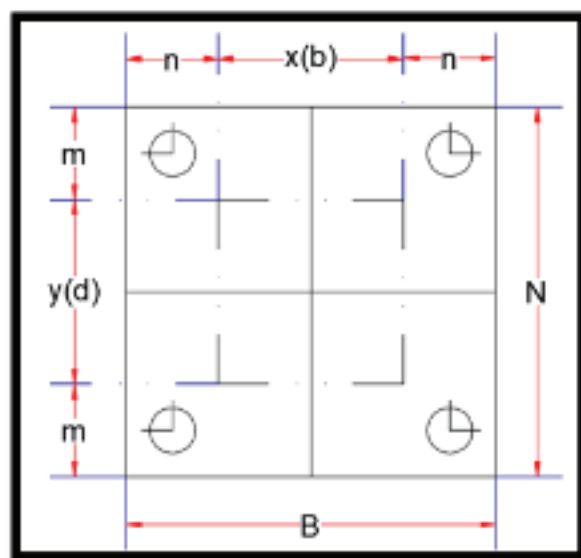
Figure 4 Column base plate dimension design
