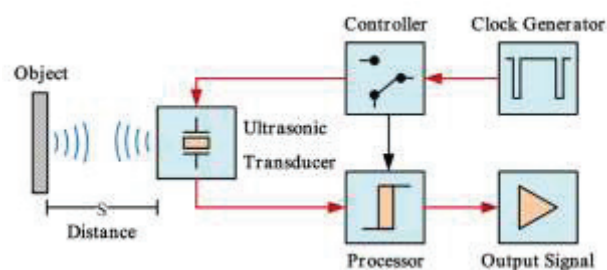
Figure 2 Operating diagram of an ultrasonic sensor
