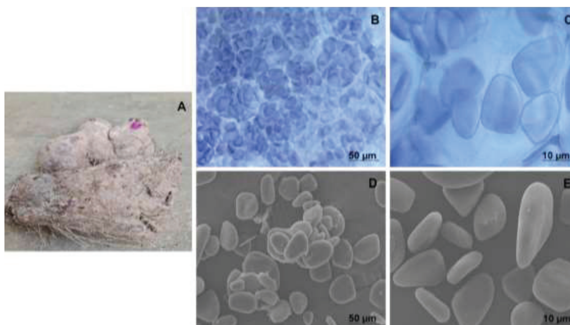
Figure 2 Morphology of yam tuber ( D. alata ) (A), starch granules in cytoplasm (B), isolated starch granules (C), starch granules visualized by SEM the scale bar 50 µm (D) and 10 µm (E)
