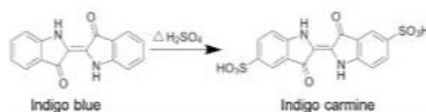
Figure 1 Indigo carmine synthesis with sulfonation
