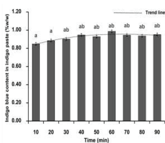
Figure 5 The effect reaction time on indigo paste sample preparation with sulfonate reaction. Different letters mean statistically significant differences at p < 0.01 .
