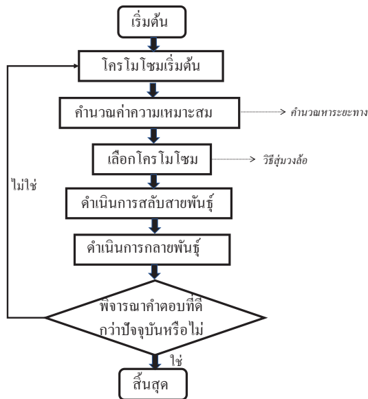
Figure 3 GA flowchart
