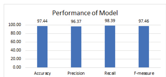
Figure 12 The results of the model performance evaluation after adjusting the appropriate parameters
