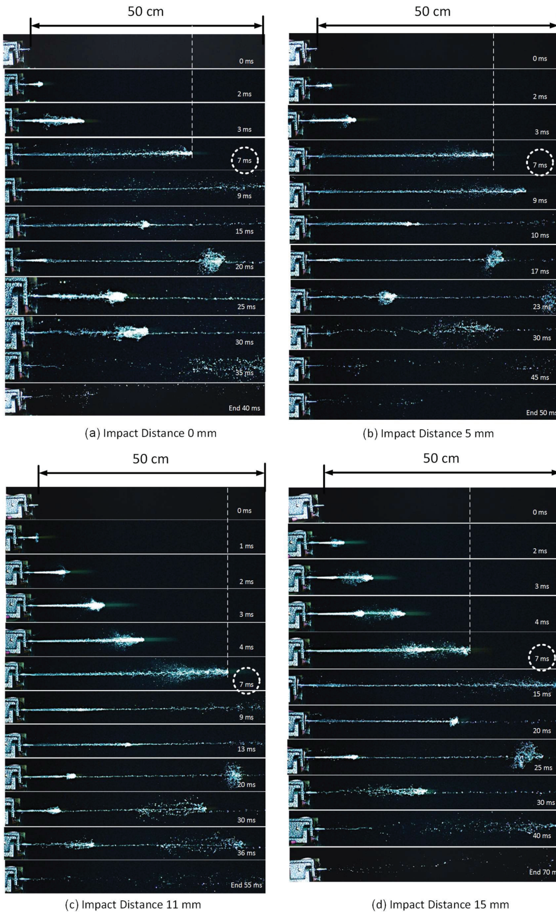
Figure 12 Visualization of the IDM jet by a high speed camera versus impact distances:
