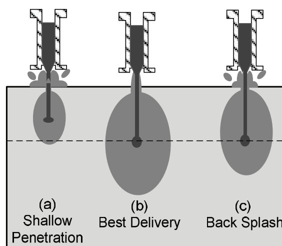
Figure 1 Drug delivery to the skin as a function of impact peak pressure (Baxter & Mitragotria, 2004)
