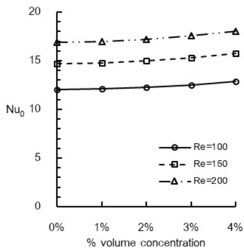
Figure 7 Stagnation point Nusselt number profiles for different volume concentrations and Re numbers at Y/B=3
