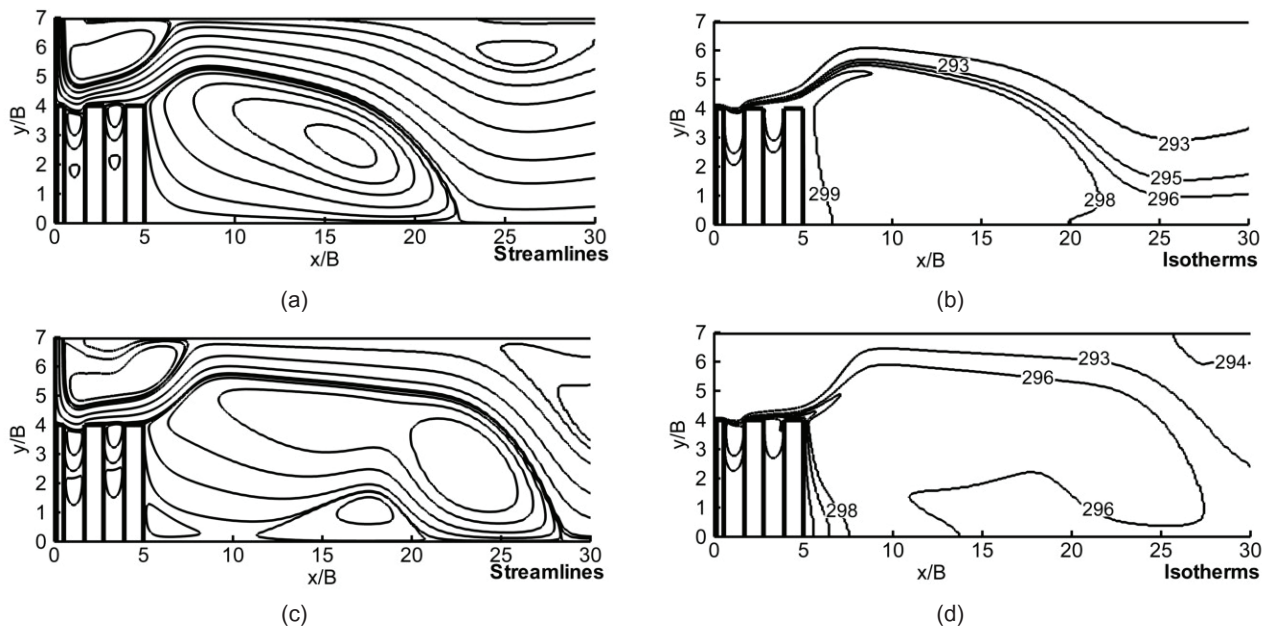
Figure 10 Streamlines and isotherms at Y/B=3 , \phi = 4\% , and different Re numbers (not to scale)
