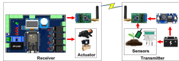
Figure 8 Wireless sensor nodes unit
