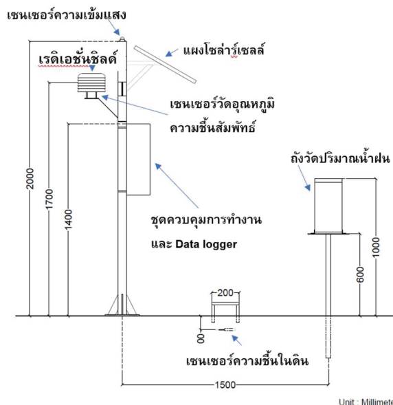
Figure 7 (a) structural drawing for installation of the Automatic in-field weather station
