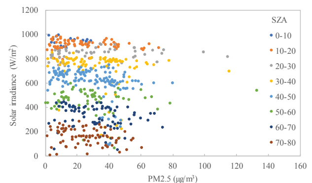
Figure 9 The relations between PM2.5 and solar irradiance at different solar zenith angles
