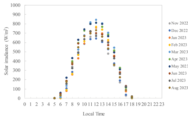
Figure 7 The variations of monthly average hourly solar irradiance
