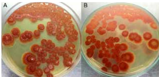
Figure 1 Colony morphology of Streptomyces sp. WPN31 in ISP2 agar with A: front and B: back mycelial images.
