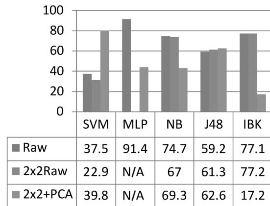
Figure 10 F-measure of models
