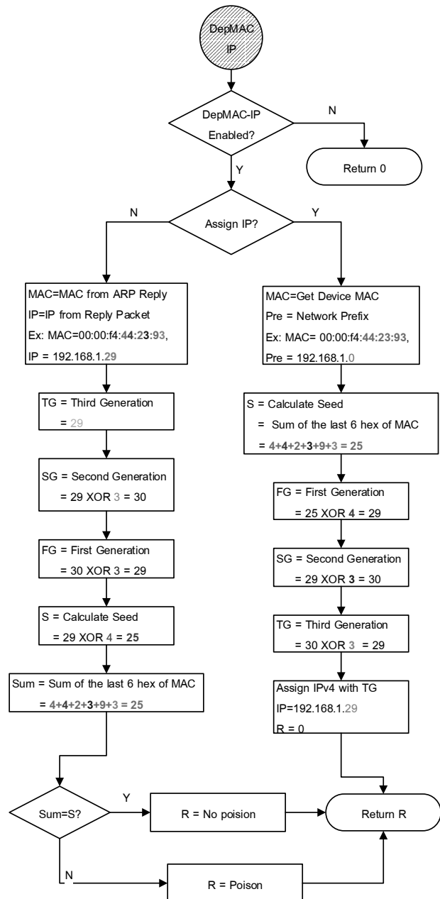
Figure 9 DepMAC-IP Algorithm
