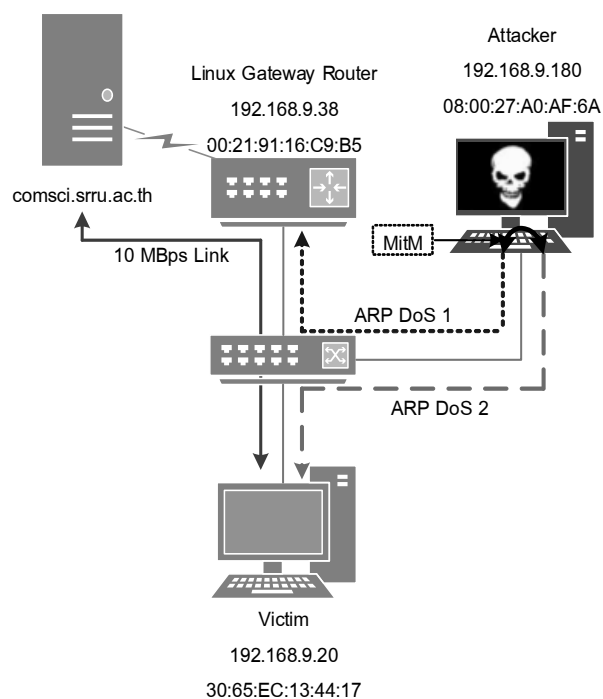
Figure 10 Experimental Testbed
