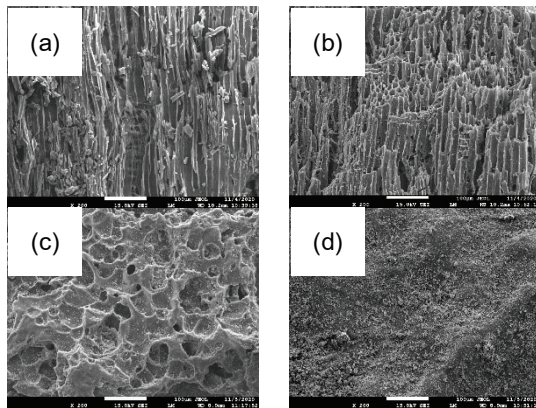
Figure 3 SEM images: (a) eucalyptus biochar (EB), (b) modified eucalyptus biochar (MEB), (c) activated carbon (AC) and (d) manganese green sand.
