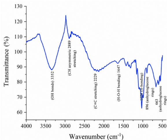
Fig. 1 FTIR spectra of cellulose extracted from corn cobs
