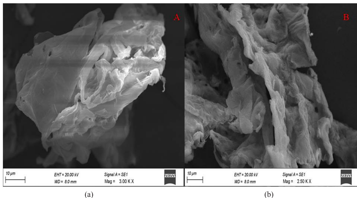
Fig. 2 SEM analysis of cellulose derived from corn cobs a) Magnification 3000x and b) magnification 2500x
