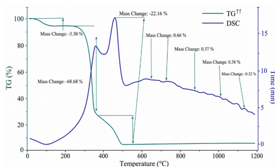
Fig. 4 Thermogravimetric analysis (TGA) thermogram of cellulose extracted from corn cobs
