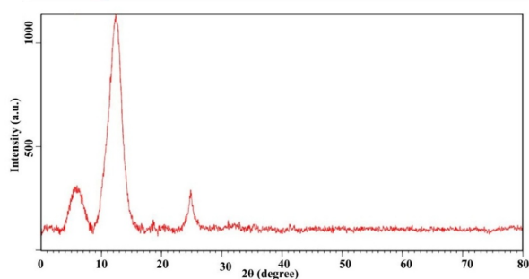
Fig. 3 X-ray diffraction (XRD) pattern of cellulose derived from corn cobs
