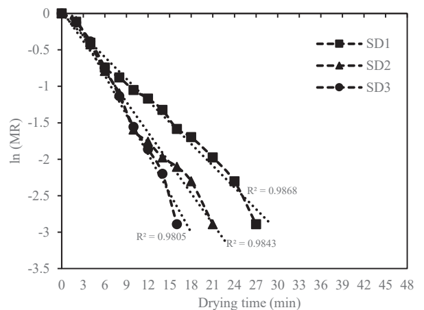
Fig. 6 Moisture ratio forecast from Fick's second law of diffusion representative of the effective diffusion coefficient, depending on the drying time at step-down MW power drying
