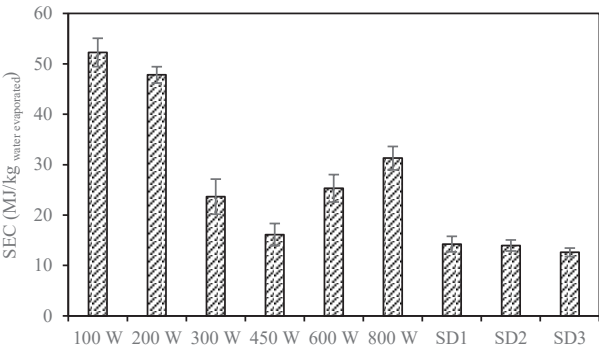
Fig. 4 Specific energy consumption of the drying process under different drying conditions
