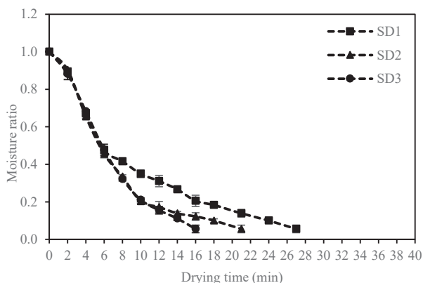
Fig. 2 Changes in the moisture ratio of pandan leaves during step-down MW drying
