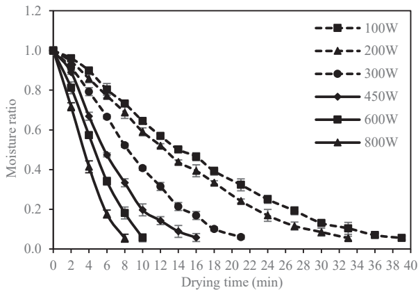
Fig. 1 Changes in the moisture ratio of pandan leaves during MW drying
