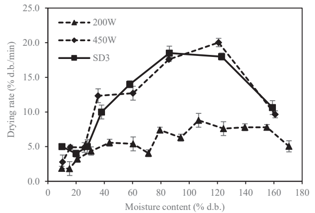
Fig. 3 Drying rate as a function of moisture content for selected drying conditions
