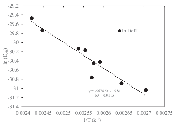
Fig. 7 Arrhenius representing the effective diffusion coefficient, dependent on the pandan leaf temperature
