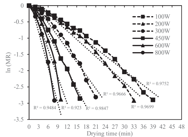
Fig. 5 Moisture ratio forecast from Fick's second law of diffusion representative of the effective diffusion coefficient, depending on the drying time at constant MW power drying
