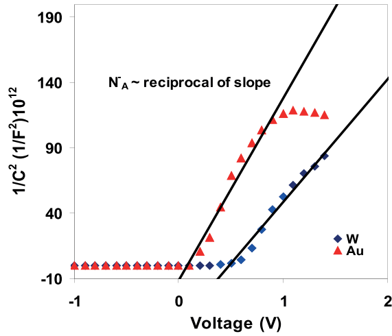
Figure 5 1/C^2 vs V_g for Au and W-gate MOS structure
