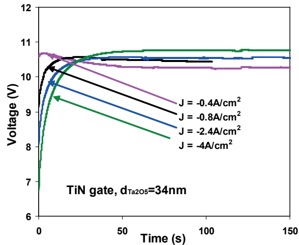
Figure 10 Voltage vs time during constant current stress for TiN gate with thicker \text{Ta}_2\text{O}_5 layer.
