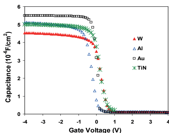
Figure 2 High-frequency C-V curves for rf sputtered oxides with different gate electrodes
