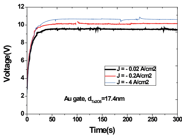
Figure 3 Voltage vs time during CCS for Au-Ta 2 O 5 -SiO 2 -Si structures with three different injected currents from the gate
