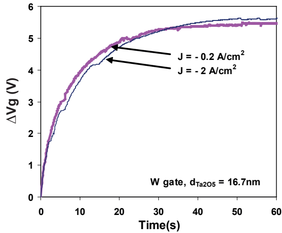
Figure 9 \Delta V_g vs time for structures with W as a gate electrode in the initial moments of stress
