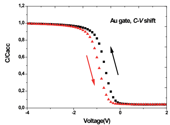
Figure 4 The hysteresis effect in MOS structures with Au gate electrode. First curve gives changes from inversion to accumulation, the second opposite direction.
