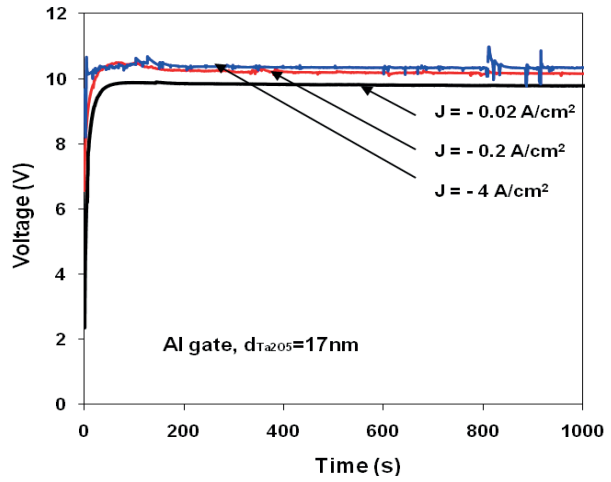
Figure 6 Long term V - t curves for Al gate oxides for three different injected currents
