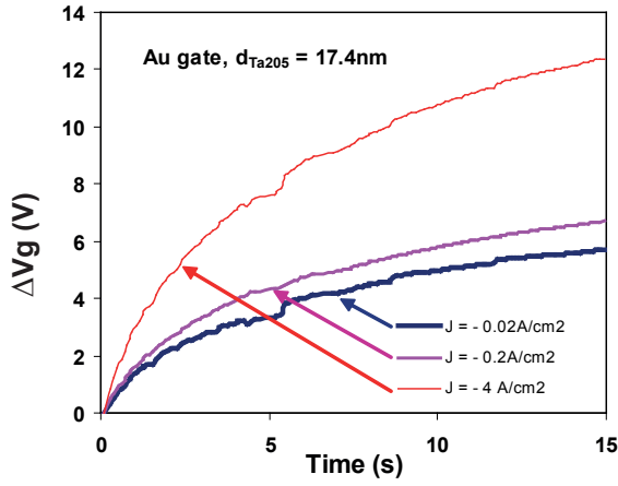
Figure 7 \Delta V_g vs time in the initial moments of stress for Au gate electrode capacitors and different injected currents
