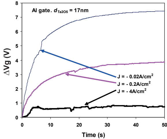
Figure 8 \Delta V_g vs time in the initial moments of stress for Al gate electrode capacitors and different injected currents.
