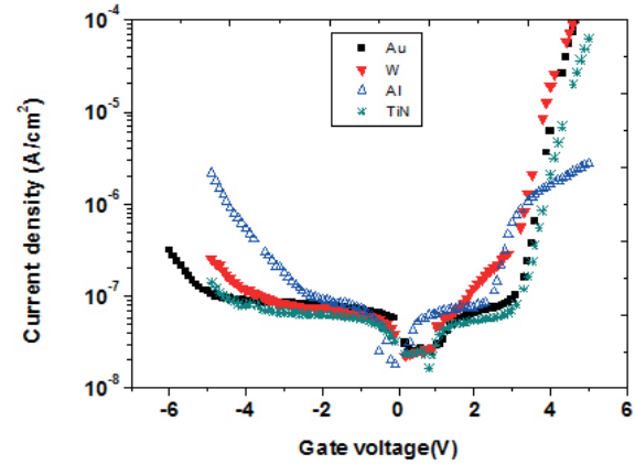
Figure 1 Leakage current density for rf sputtered Ta 2 O 5 films with different gate electrodes
