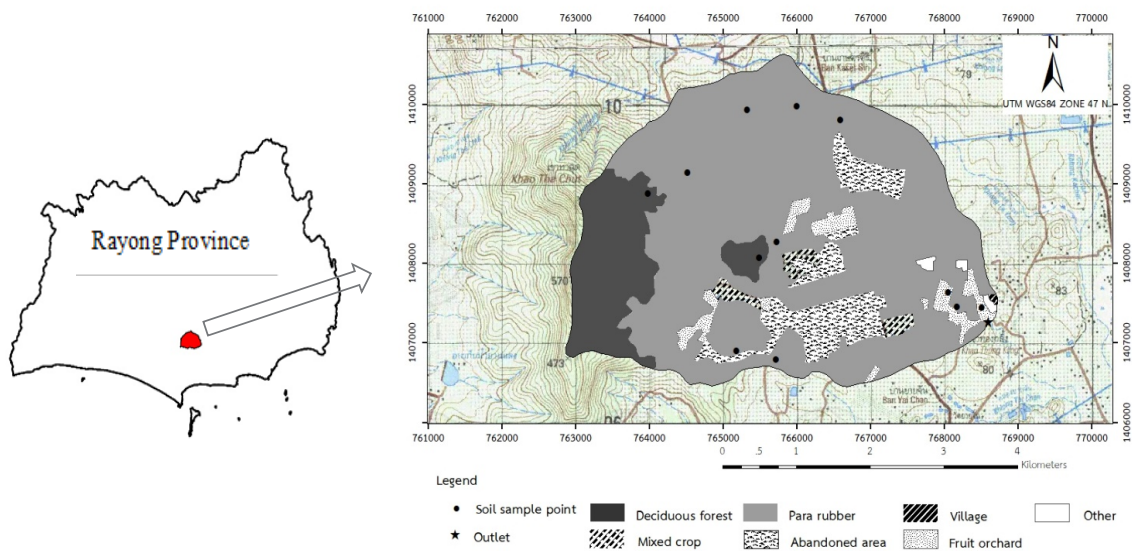
Figure 1 Study site, land use, and sample points in Eastern Coast subwatershed, Rayong province. Source: Modified from Land Development Department (2013)
