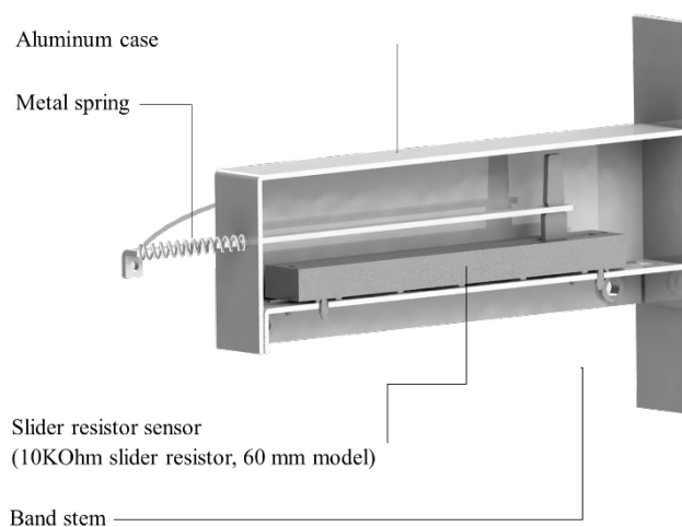
Figure 2 3D model of the Sensor unit.
