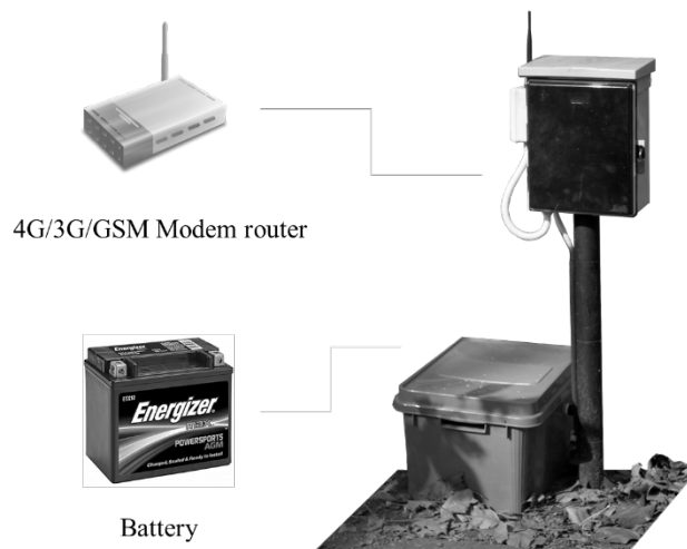
Figure 4 Gateway.
