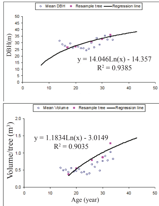
Figure 6 Growth model of treeheight, DBH and stem volume of Pinus kesiya plotted against stand age in northern highland watershed.
