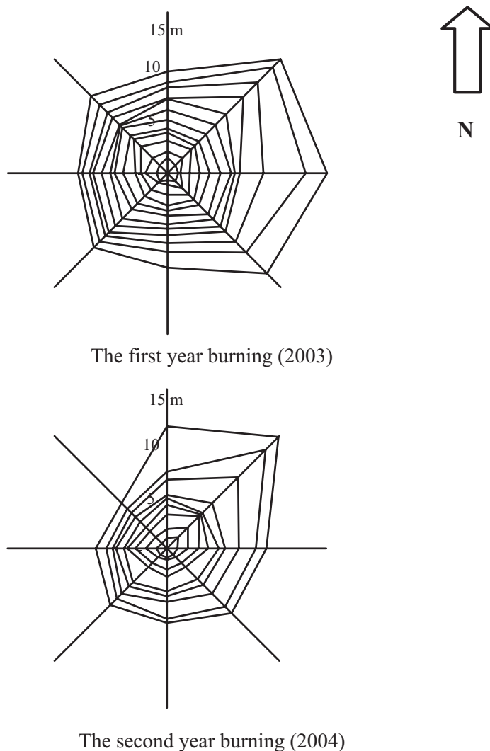
Figure 1. Burn patterns of the first and the second year burning in the dry deciduous dipterocarp forest
