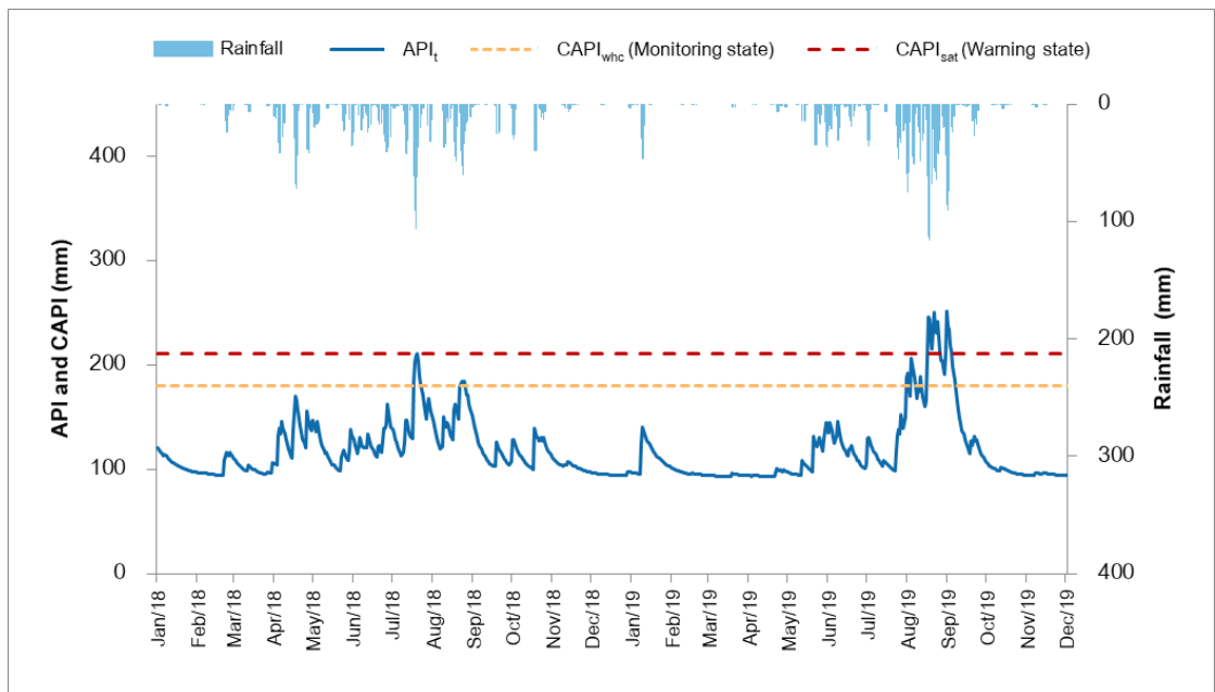
Figure 1 Influences of rainfall and antecedent precipitation index to overland flow generation in forest watershed during January 2018 to December 2019.
