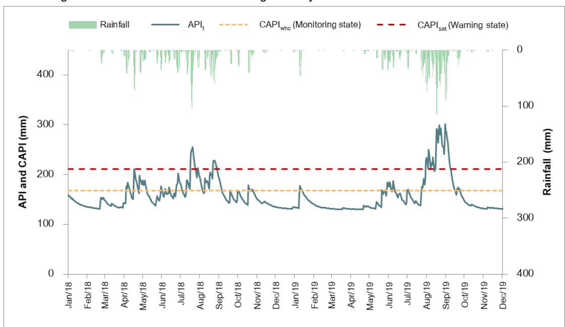
Figure 2 Influences of rainfall and antecedent precipitation index to overland flow generation in agricultural watershed during January 2018 to December 2019
