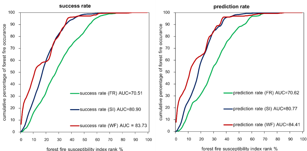
Figure 6: Success rates (left) and prediction rates (right) of FR, SI and WF methods
