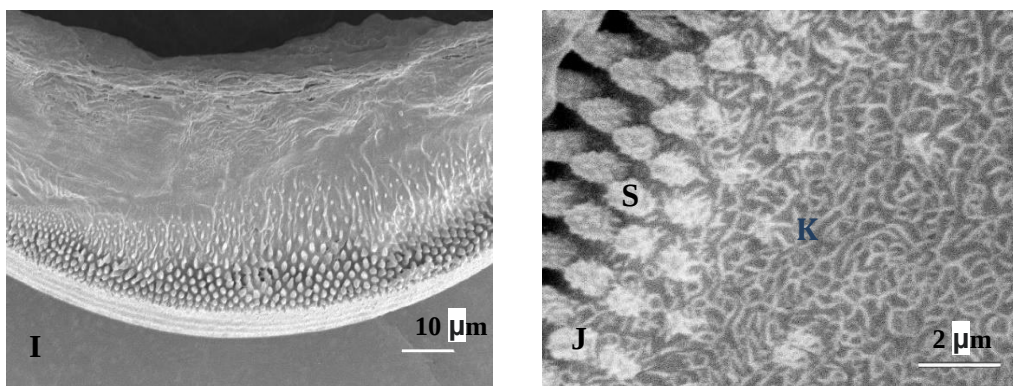
Figure 3. Several ultrastructural aspects observed in juvenile Hyriopsis bialatus using scanning electron microscopy (SEM): I-J: 10 days old juveniles showing anterior periostracum (AP); initial glochidia shell (IS); posterior periostracum (PP); growth lines of periostracum (GL); hard periostracum (HP); cuticle buds (B); pores in the internal calcareous layer (PO); spines (S) and keratin fibers (K).
