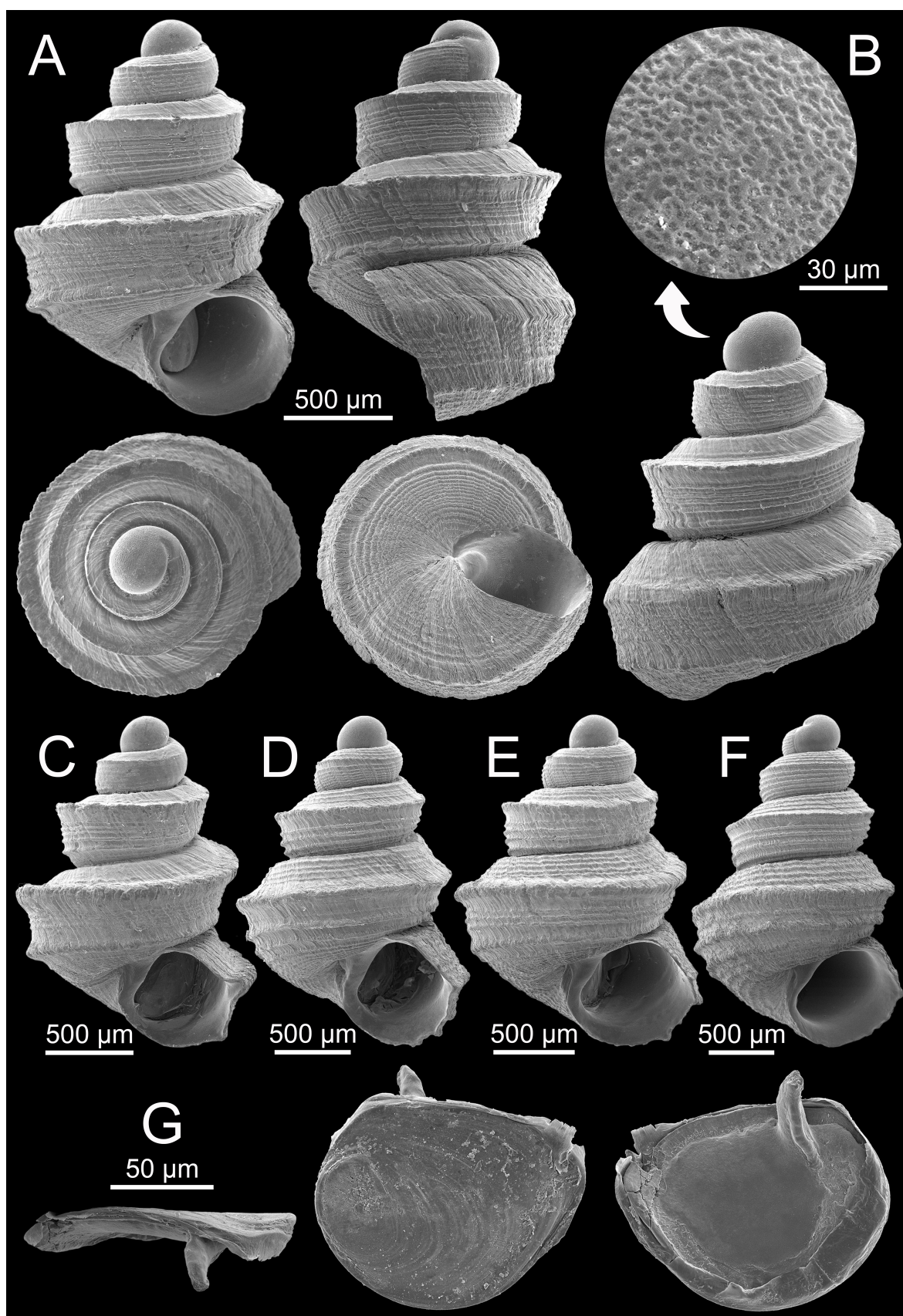
FIGURE 3. Scanning electron micrographs of Georissa chatra sp. nov. A. holotype CUMZ 15265 from Wat Khao Pathawi, Uthai Thani. B, C. paratype CUMZ 15266 from the type locality, ( B ) close-up view of protoconch and ( C ) entire shell in apertural view. D–G specimen CUMZ 15270 from limestone hill near Wat Si Uthum Phon, Nakhon Sawan, ( D–F ) entire shells in apertural view and ( G ) operculum with lateral view, and outer and inner surface views, respectively.
