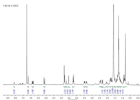
Figure 3 ^1\text{H} NMR (300 MHz, \text{CDCl}_3 ) spectrum of fraction 25/26
