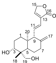
Figure 4 Structure of 14-deoxy-11,12-didehydroandrographolide
