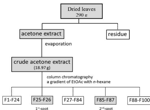
Figure 1 Schematic summary of the acetone extraction and chromatographic separation of bioactive compounds from the leaves of Andrographis paniculata
