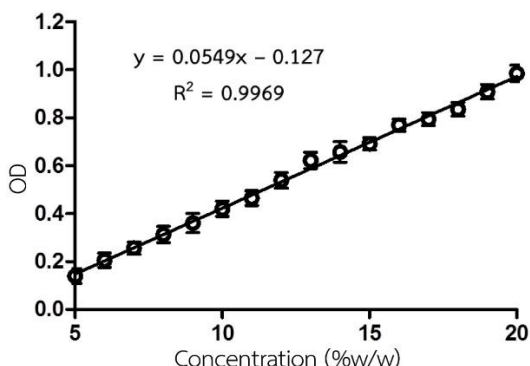
Figure 8 Standard curve of lactones at various concentration as 5-20 %w/w
