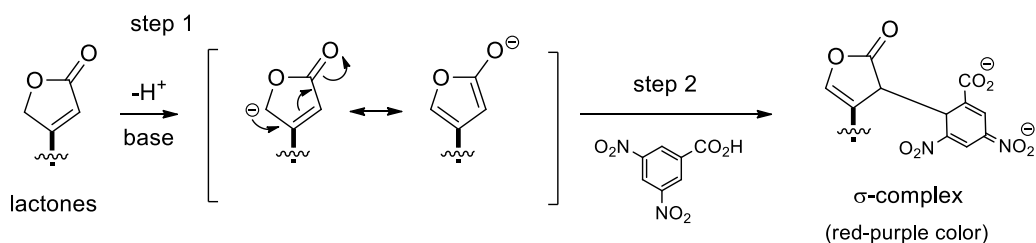
Figure 7 Kedde's reaction assay with lactones
