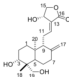
Figure 6 Structure of andrographolide
