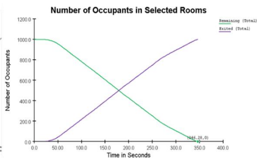
Figure 14 An illustration of the 5 th scenario emergency (left); Number of evacuees at each period (right)
