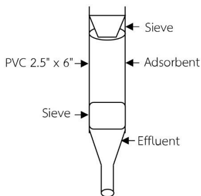
Figure 1 Equipment of adsorption experiment
