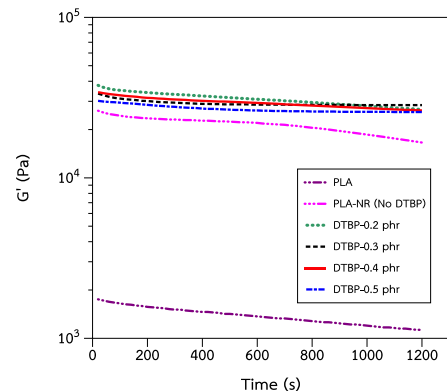
Figure 5 Storage modulus as a function of time for PLA, PLA-NR, and PLA-g-NR with different DTBP contents.
