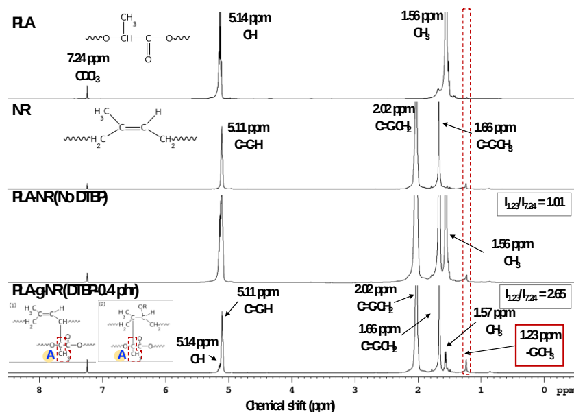
Figure 3 ^1\text{H} -NMR spectra of PLA, NR, PLA-NR, and PLA-g-NR with 0.4 phr DTBP.
