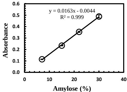
Figure 4 Calibration spectrum (left) and curve (right) of iodine binding method using rice starch standard
