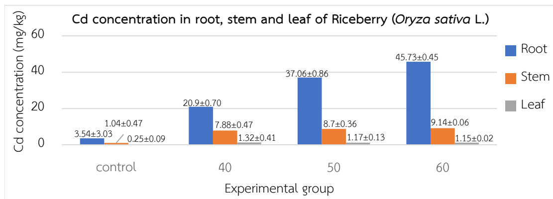
Figure 2 Cadmium concentrations in root, stem and leaf of Riceberry ( Oryza sativa L.) after 3 months of the experiment
