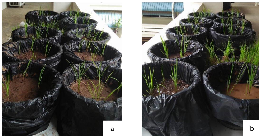
Figure 1 The experimental group containing cadmium ( \text{Cd}^{2+} ) in soil (a) and the experimental group containing lead ( \text{Pb}^{2+} ) in soil (b)
