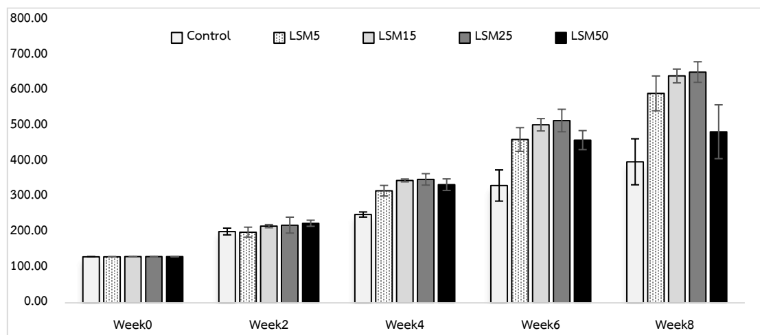
Figure 1 Growth performance of Nile tilapia fed diet containing different levels of longan seed meal (LSM) for 8 weeks
