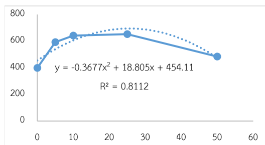
Figure 2 Effect of different levels of protein replacement by LSM with broken rice meal on final weight of tilapia. This estimate was calculated using the polynomial regression.
