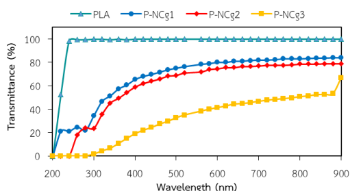
Figure 6 Light transmission of PLA film and PLA/NR/Cg blend films
