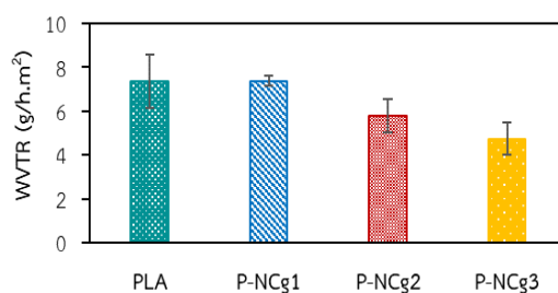
Figure 7 Water vapor transmission rate of PLA film and PLA/NR/Cg blend films
