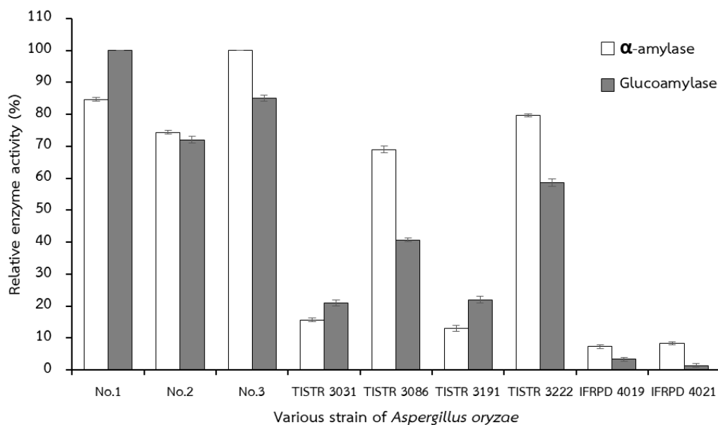
Figure 2 Relative enzyme activities of \alpha -amylase and glucoamylase from various strains of Aspergillus oryzae
