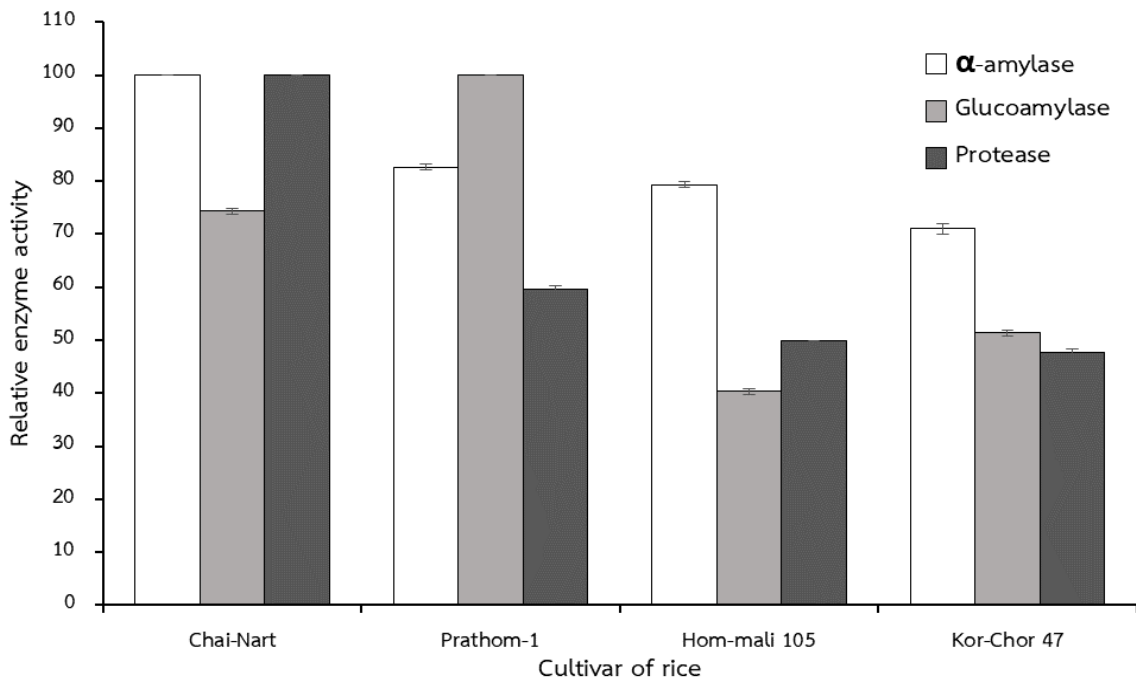
Figure 4 Relative enzyme activities of Aspergillus oryzae strain No.3 on various rice cultivars.
