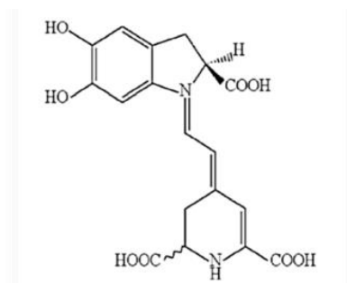
Figure 1 Betacyanin structure
