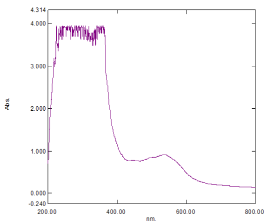
Figure 3 Maximum absorption wavelength of the extract from white dragon fruit peel
