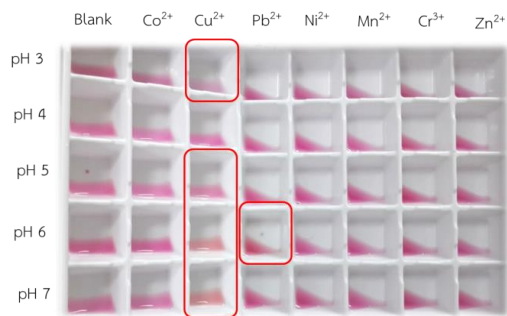
Figure 4 Interaction of reagent extracted from white dragon fruit peels and metal ions ( \text{Co}^{2+} , \text{Cu}^{2+} , \text{Pb}^{2+} , \text{Ni}^{2+} , \text{Mn}^{2+} , \text{Cr}^{3+} , and \text{Zn}^{2+} )
