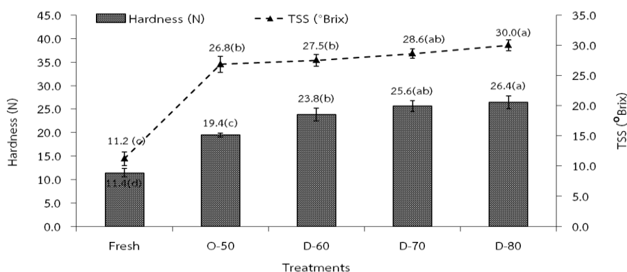
Figure 5 Changes in hardness values and total soluble solid (TSS) of fresh melon, osmosis melon and osmosis melon drying at 60, 70, and 80 °C. [Different letters above the data bars indicate significant difference treatment (DMRT, p < 0.05 )]
