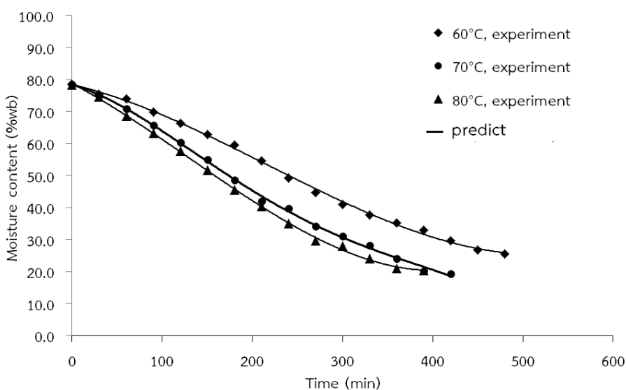
Figure 1 Effect of drying temperature on moisture content versus time during drying of melon osmosis at 60, 70, and 80 °C.
