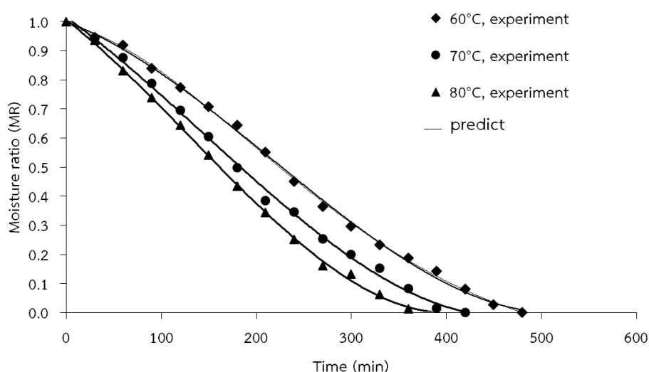
Figure 2 Effect of drying temperature on moisture ratio versus time during drying of melon osmosis at 60, 70, and 80 °C.
