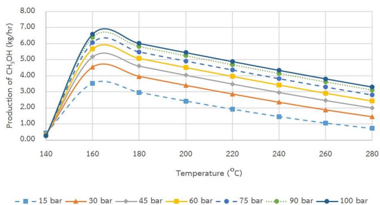
Figure 6 Effects of temperature and pressure on methanol production
