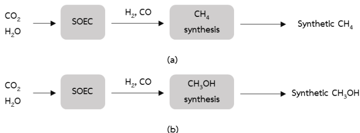
Figure 1 Process block diagrams
