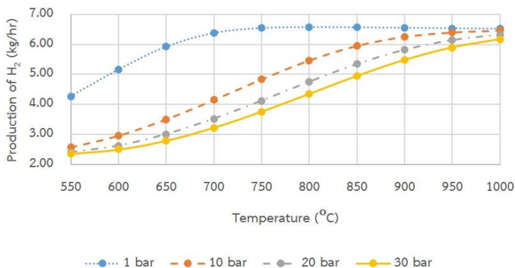
Figure 2 Effects of temperature and pressure on SOEC
