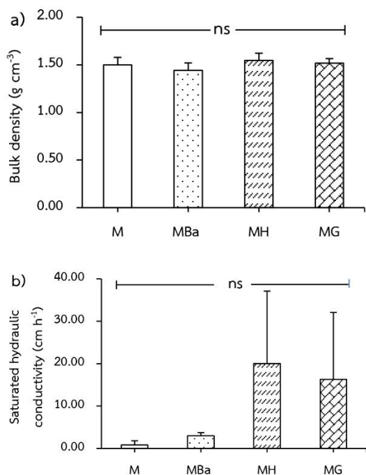
Figure 3 Bulk density (a) and saturated hydraulic conductivity (b) of rubber growing soil under different rubber-based intercropping systems [M = rubber monoculture, MBa = rubber-bamboo, MH = rubber- Hopea odorata , MG = rubber- Gnetum gnemon ; bar = S.D.; ns = not significant difference ( p > 0.05 ) by DMRT]
