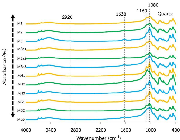
Figure 5 FTIR spectra of rubber growing soil under different rubber-based intercroppings. The band assignments are 2,920\text{ cm}^{-1} for aliphatic-C, 1,630\text{ cm}^{-1} for carboxylic-C, 1,160\text{ cm}^{-1} for polysaccharides and 1,080\text{ cm}^{-1} for quartz or cellulose C-O. (M1-3 = rubber monoculture, MBa1-3 = rubber-bamboo, MH1-3 = rubber- Hopea odorata , MG1-3 = rubber- Gnetum gnemon )
