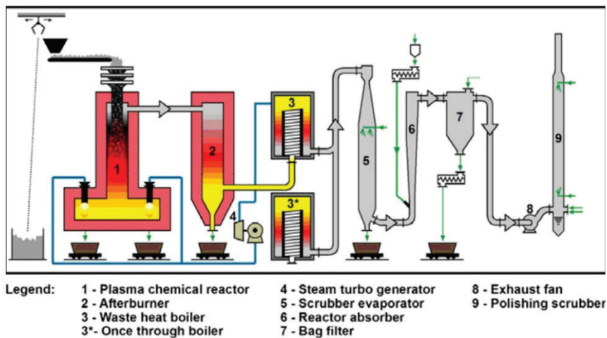
Figure 3 Illustration of the plasma gasification melting plant [23]
