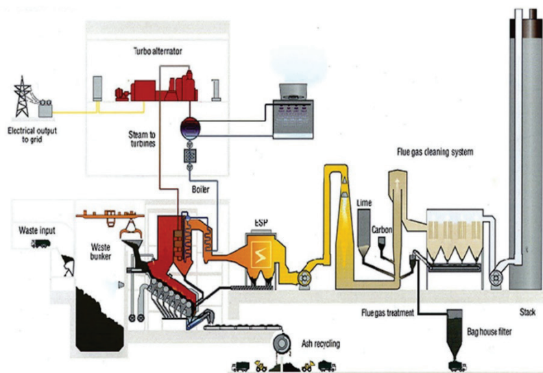
Figure 2 Waste incineration plant using heat to generate electricity [3].
