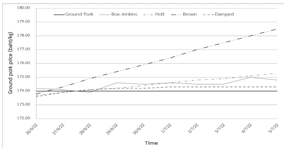
Figure 7 Comparison of the first dataset of daily ground pork price with forecast values
