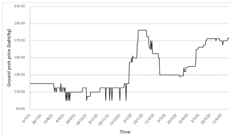
Figure 1 Run plot of the ground pork price from July 6, 2021, to June 25, 2022
