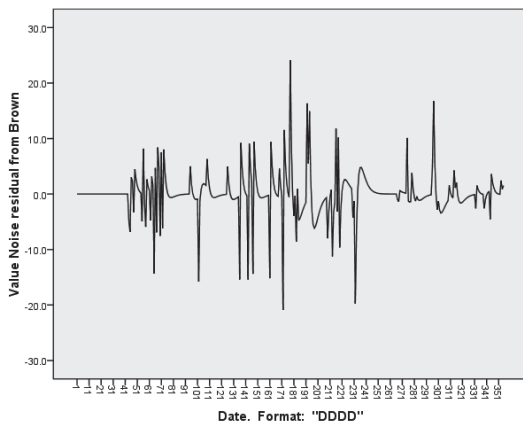
Figure 5 Errors from Brown's exponential smoothing method
