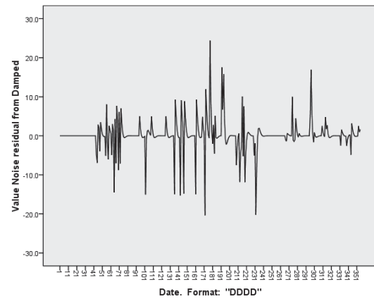
Figure 6 Errors from damped trend exponential
