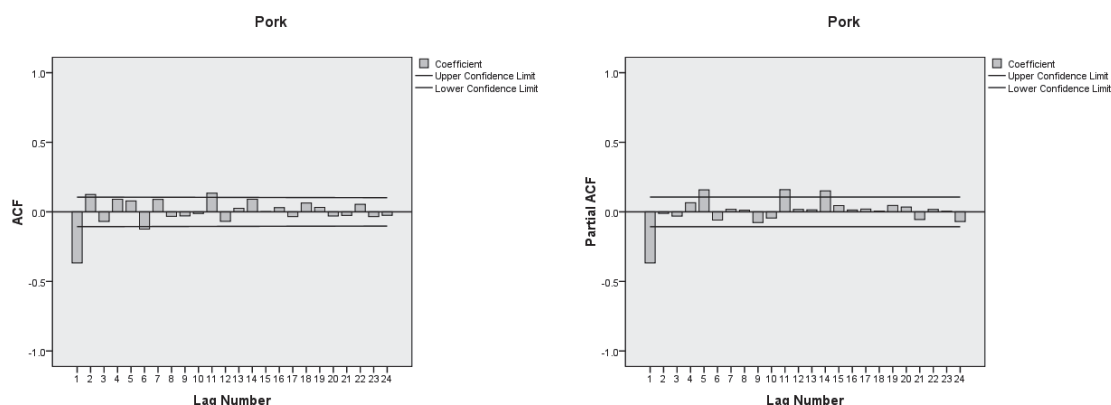
Figure 2 ACF and PACF of the first difference, d = 1 , of the ground pork price
