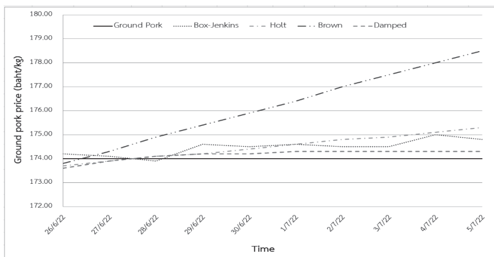
Figure 8 Comparison of the second dataset of daily ground pork price with forecast values
