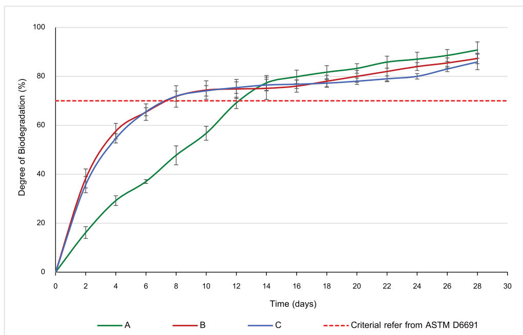
Figure 2 Biodegradation percentages of cellulose chromatography grade
