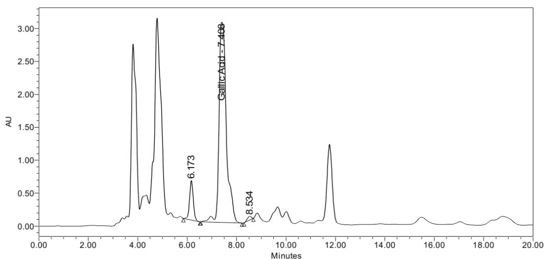
Figure 1 Chromatogram of Triphala water extract
