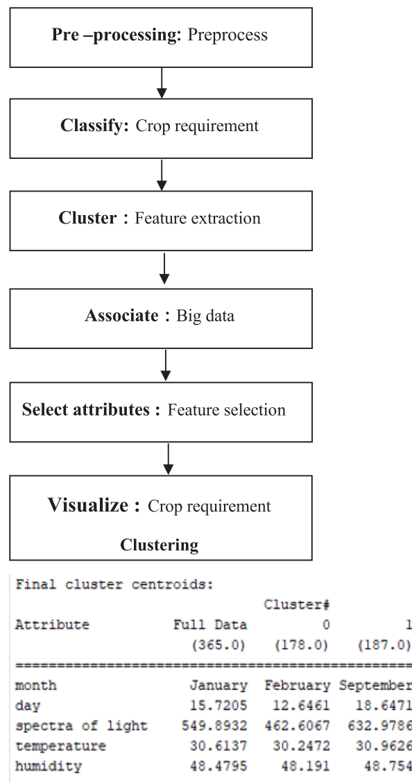
Figure 5 Processed with k-means clustering method.
