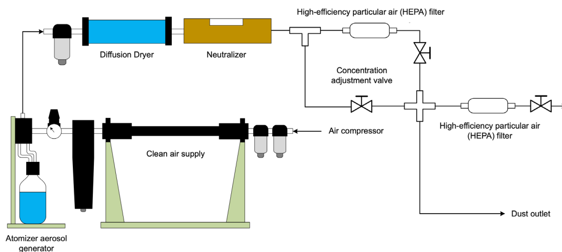
Figure 5 Schematic diagram for testing aerosol generation
