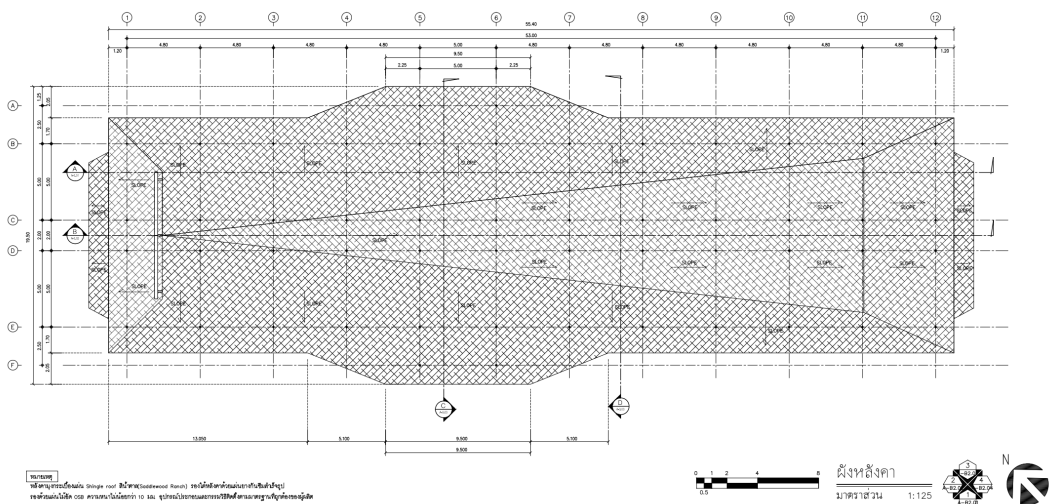
Figure 2 Roof plan of C-Dormitory, Chiangrai College.
